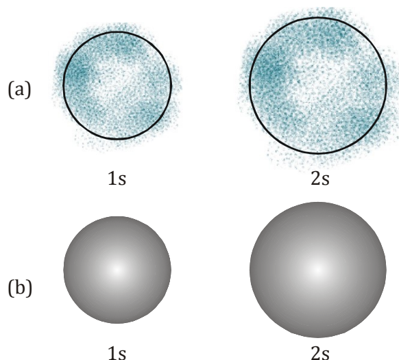
(a) Probability density plots of 1s and 2s atomic orbitals. The density of the dots represents the probability density of finding the electron in that region. (b) Boundary surface diagram for 1s and 2s orbitals.
