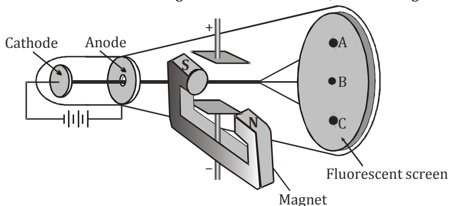
The apparatus to determine the charge to the mass ratio of electron
