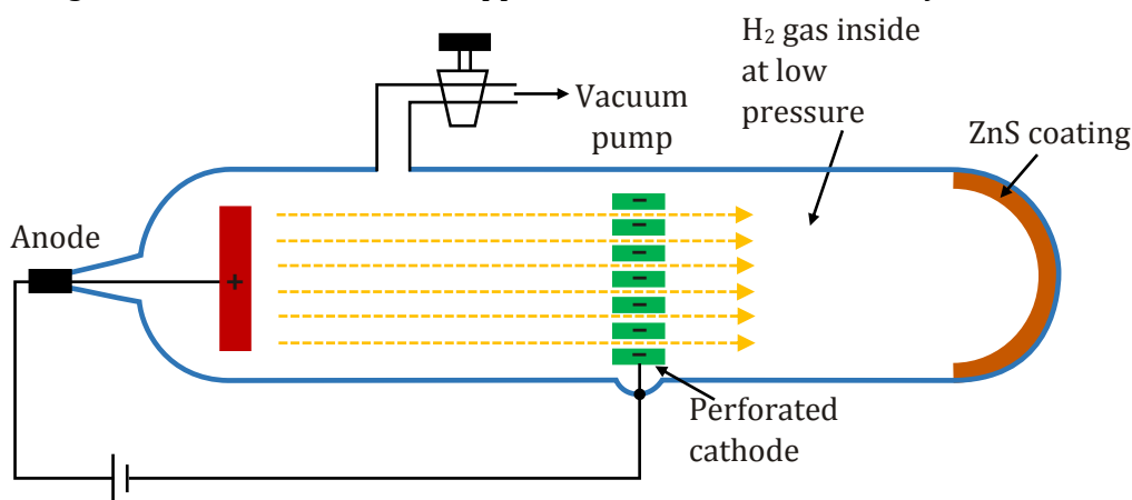
Positive Rays or Canal Rays
